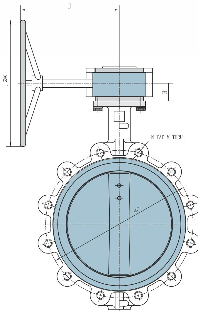
Disassembly Gear Operator
